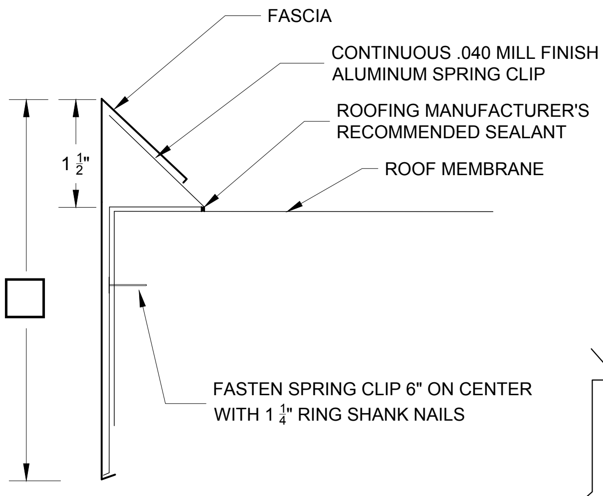
CLEAT DETAIL
